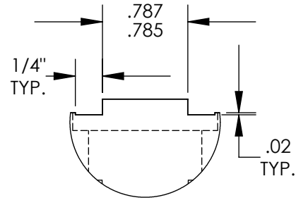
DETAIL B SCALE 1 : 1.25
