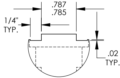
DETAIL B SCALE 1 : 1.25
