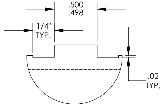
DETAIL B SCALE 1.5 : 1
