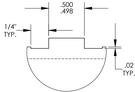
DETAIL B SCALE 1.5 : 1
